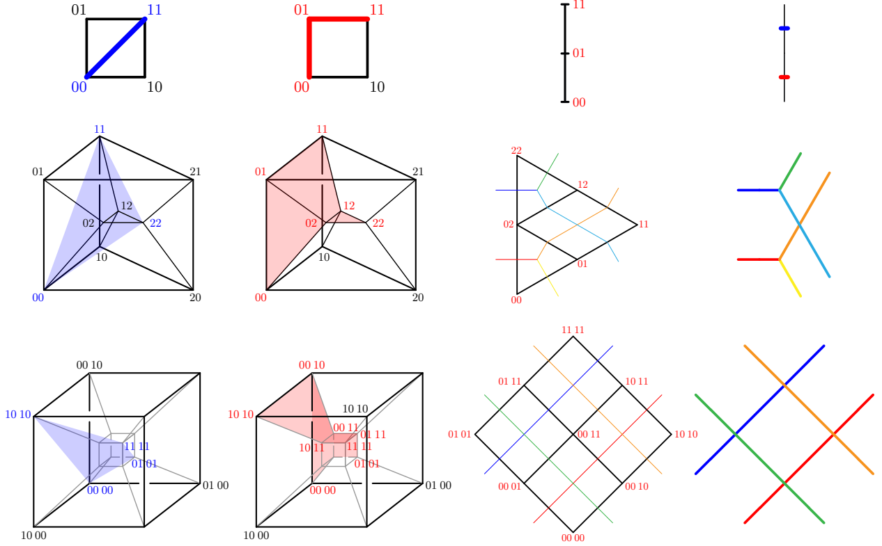
Figure 1: Cellular diagonals of the segment (top), the triangle (middle) and the square (bottom). For each of them, we have represented the thin diagonal of P (left, in blue) and a cellular diagonal of P (mid. left, in red) both represented in P \times P , the associated polytopal subdivision of P (mid. right) and the common refinement of the two copies of the normal fan of P (right) both represented in P .
