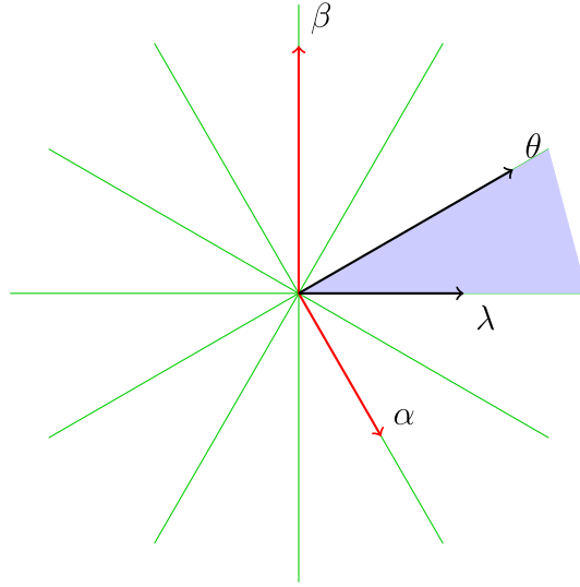
Fig. 3. G_2 root system.
