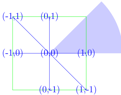
Fig. 5. Steps in octant.
