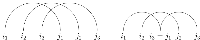
Fig. 6. A 3-crossing and an enhanced 3-crossing.
