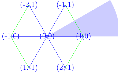
Fig. 4. Steps in weight lattice.
