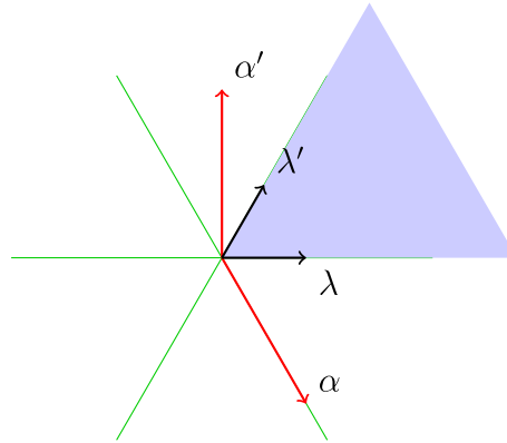
Fig. 7. A_2 root system.
