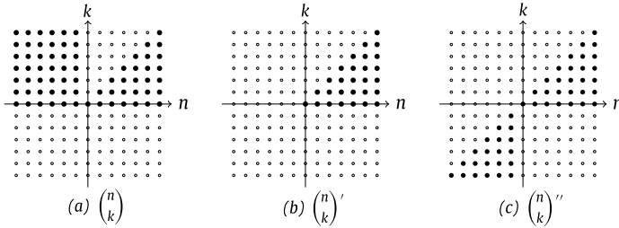
Fig. 2. Supports of some variants of the binomial coefficient.
