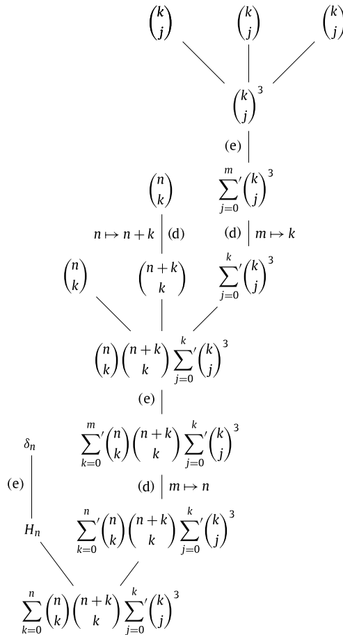
Fig. 1. Construction of a binomial sum. The last step replaces the directed sum by a usual sum in order to have nonzero values for n \geq 0 only.
