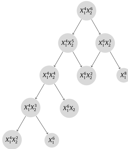
Fig. 8. Tree structure of the reduction by S_2 .
