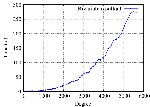
Fig. 12. Timings in magma.
