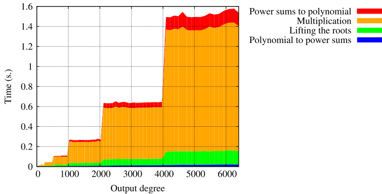
Fig. 11. Detailed timings for our algorithm.
