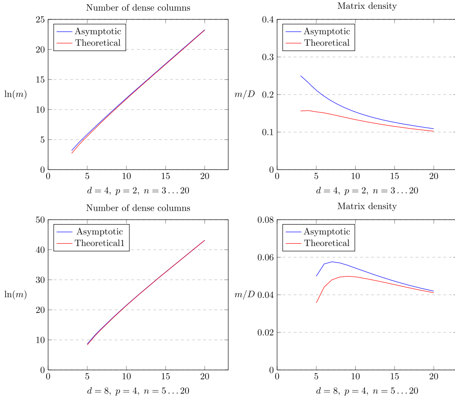
Fig. 1. Comparison of our asymptotic formulae against the theoretical number of dense columns and matrix density for generic critical point systems with parameters (d, p, n) .
